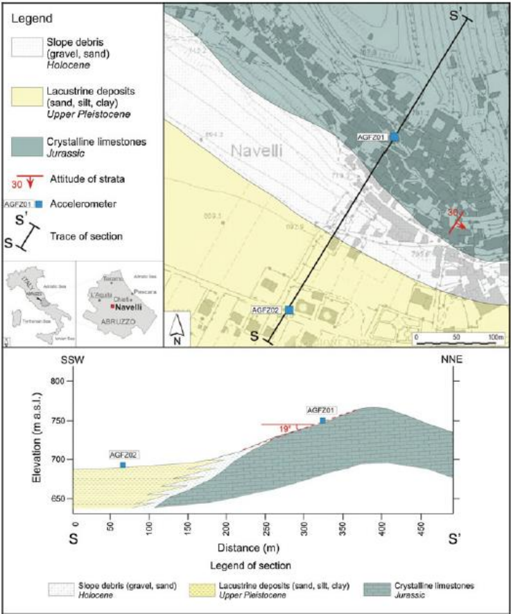
Fig. 7 Geological map and section for Navelli
