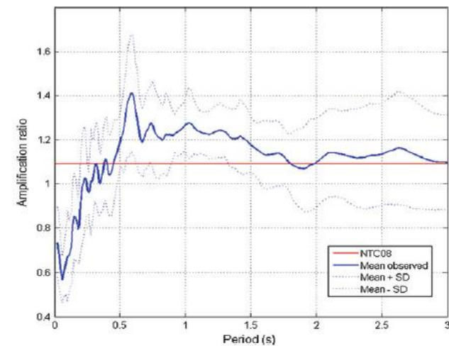
Fig. 6 Comparison between code provisions ratio (red) and observed amplification ratio (blue) in Castelnovo
