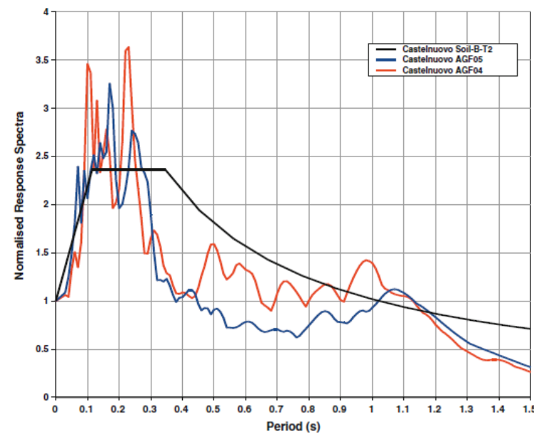
Fig. 5 Normalised Response spectra of the M 5.1 event of April 9, 2009 recorded at two sites in Castelnovo compared with code provision
