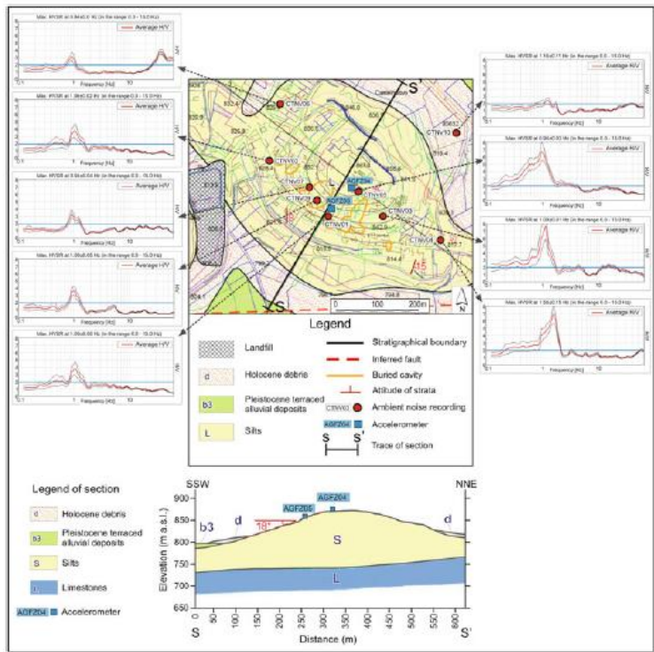
Fig. 2 Geological map and section for Castelnovo (modified from Gallipoli et al. 2011)
