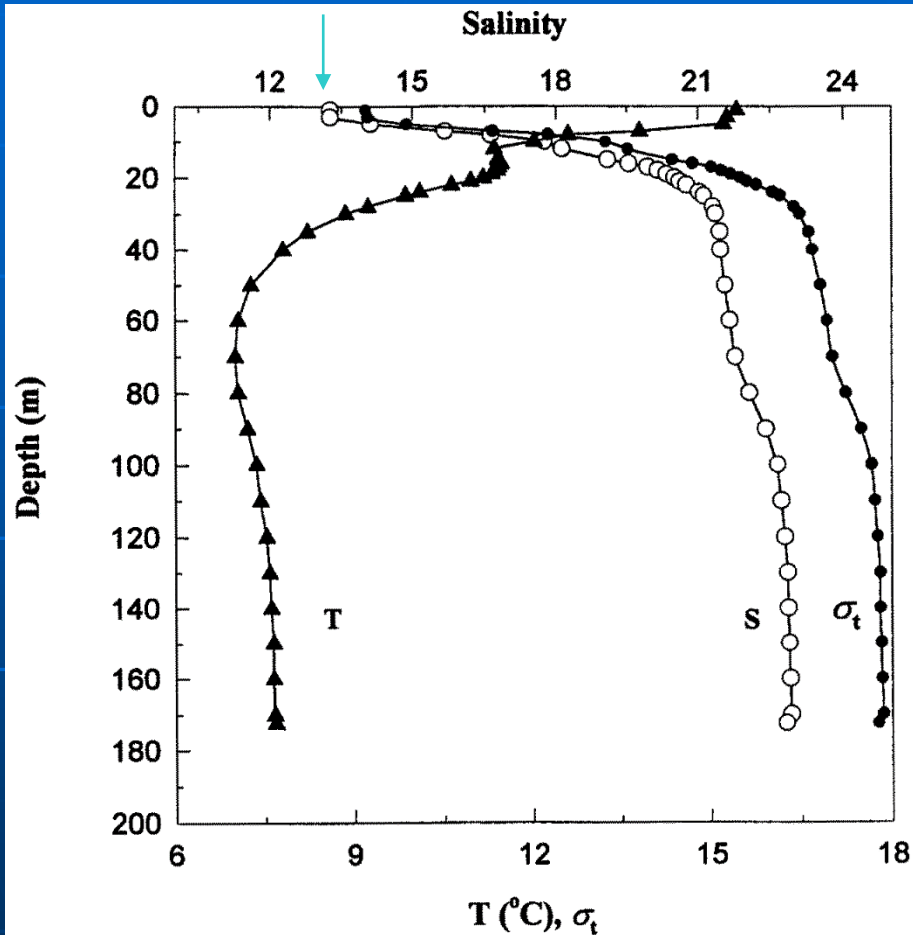
Fig. 1. Temperature, salinity and density profiles for the Framvaren Fjord waters.
