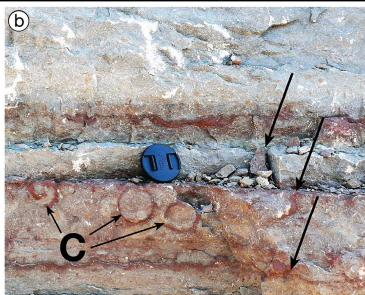
Orhtoceras limestone (Sweden) depositen in a large epicratonic sea that in the Ordovician occupied a large portion of the Baltic Shield. The succession (a) is very condensed and few tens of meters thick. It is charcaterized by numerous hardgrounds (arrows in b). Orthoceras shells are marked with letter «C». From James and Jones, 2015.
