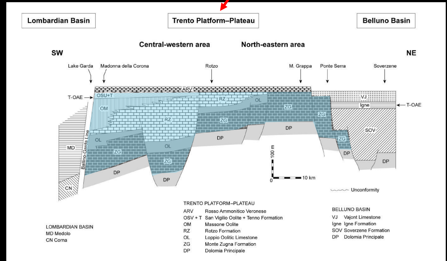
The Early Jurassic shallow water units of the Trento Platform (blue). From Masetti et al., 2011, modified
