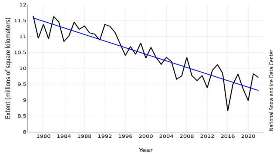
Average Monthly Arctic Sea Ice Extent November 1978 - 2022
