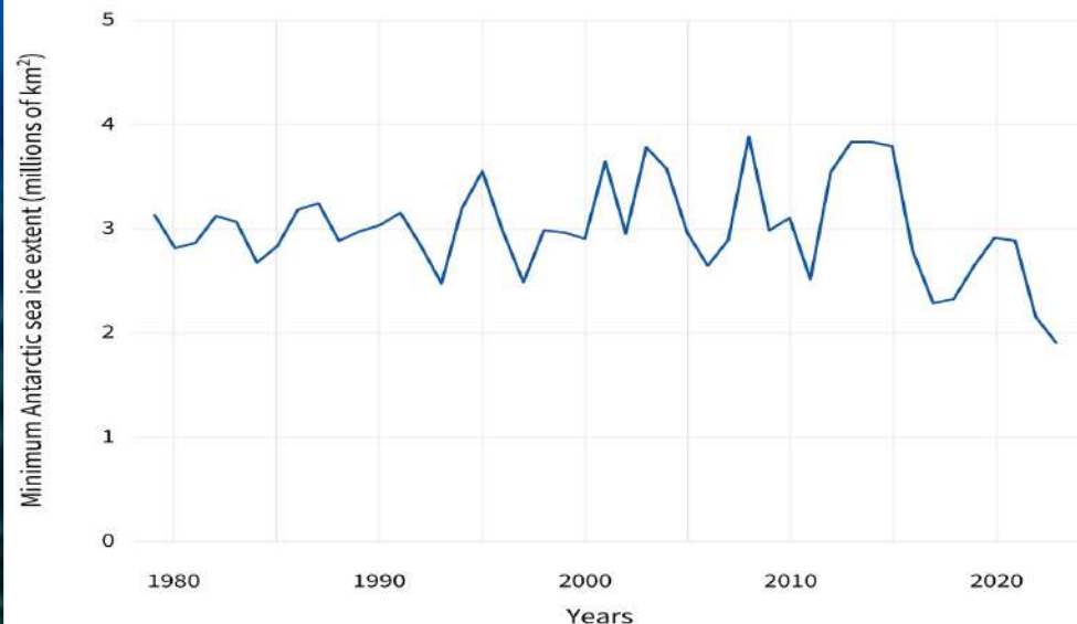
ANTARCTIC SEA ICE YEARLY MINIMUM
