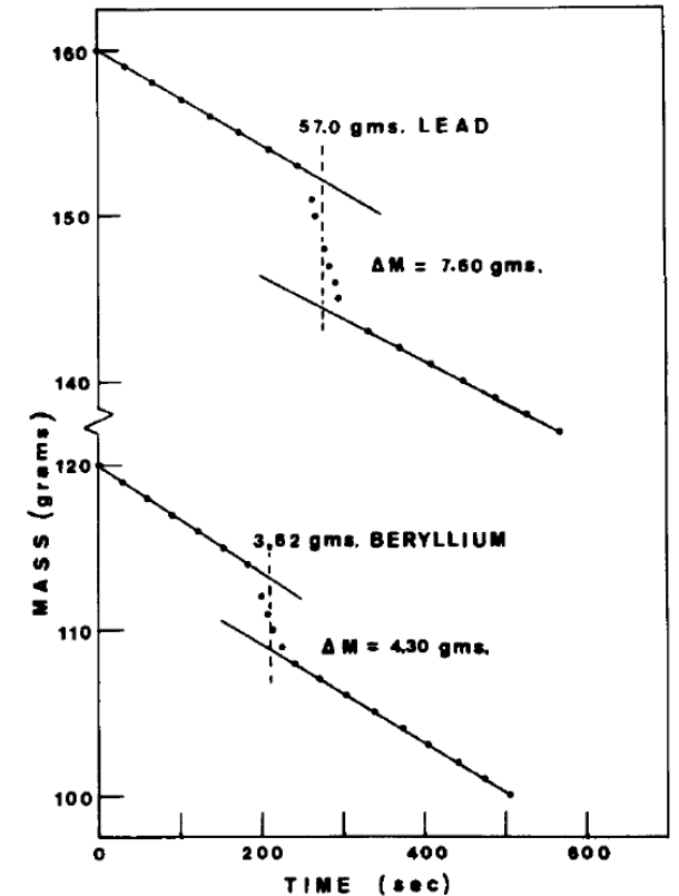
Fig. 4. Plots of the data which show the mass of the sample cup assembly plus LN 2 as a function of time for the heat capacity measurements for lead (upper) and beryllium (lower). The background rates have been extrapolated into the region where the cooling of the sample occurred. The mass of the nitrogen boil off \Delta m and the mass of each sample are shown for the two measurements.
