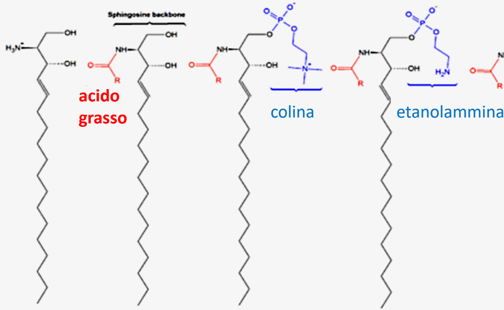
singosina ceramide
