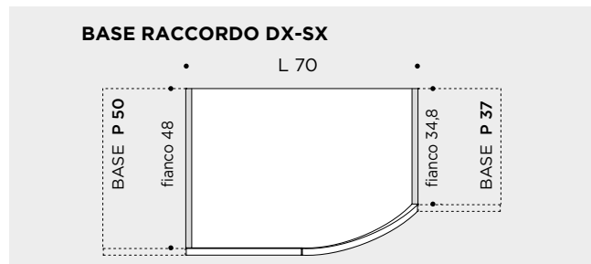
Base raccordo 2 ante 1 anta Fusion dx-sx
