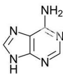
A Adenine \text{C}_5\text{H}_5\text{N}_5
