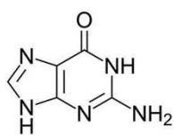
G Guanine \text{C}_5\text{H}_5\text{N}_5\text{O}
