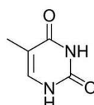
T Thymine \text{C}_5\text{H}_6\text{N}_2\text{O}_2
