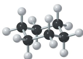
chair conformation
