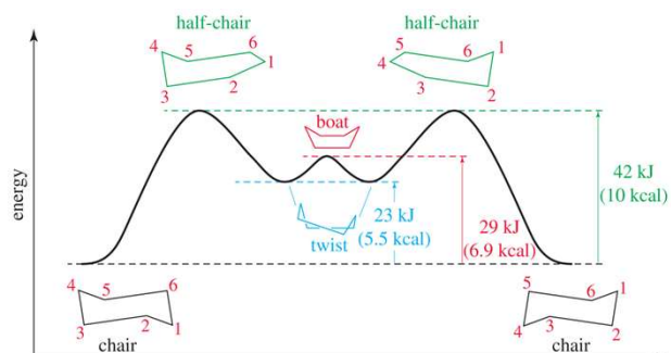
boat conformation
