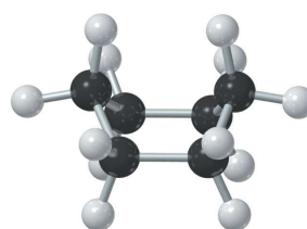
boat conformation
