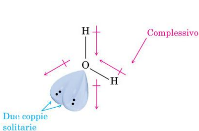
Acqua, \text{H}_2\text{O} ( \mu = 1.85 \text{ D} )
