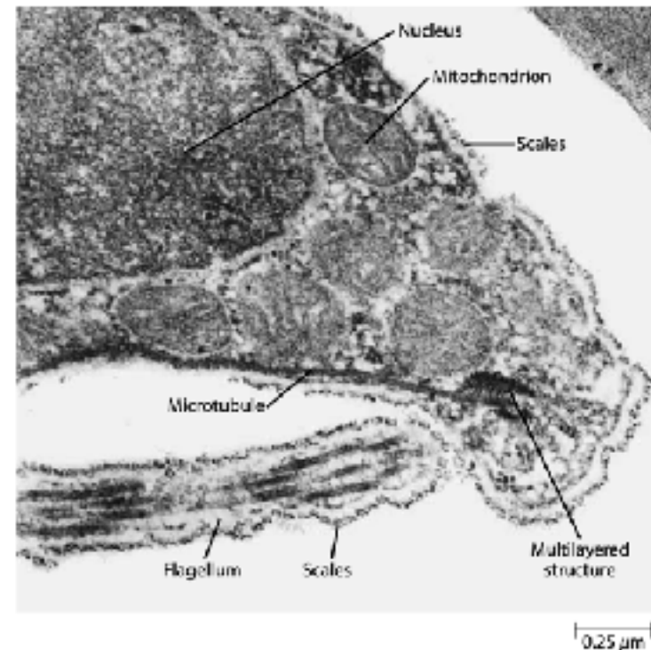
15-33 Charophyte asymmetrical flagellar root system
