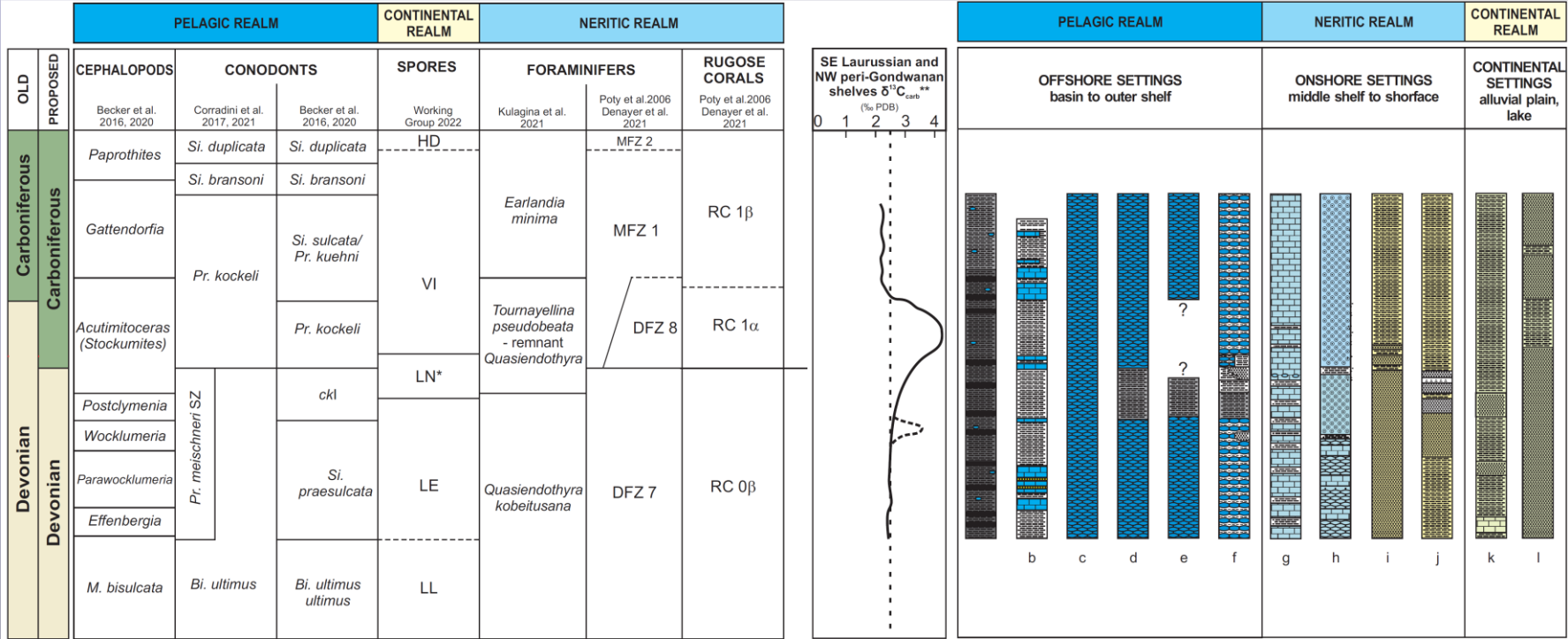
LIMITE DEVONIANO/CARBONIFERO (in progress)
