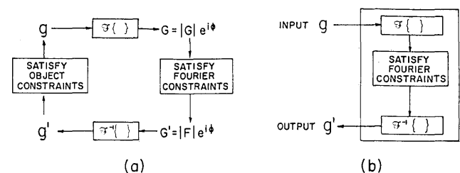
Fig. 1. (a) Block diagram of the error-reduction approach; (b) block diagram of the system for the input-output concept.
