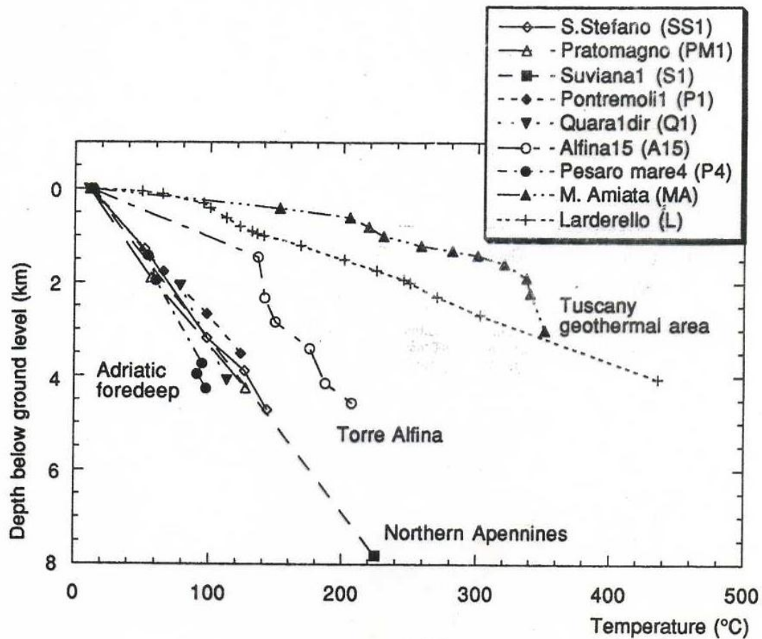
Figure 7.5 Temperature distribution with depth in the Northern Apennines. The thermal gradients increase from the Adriatic foredeep areas towards the inner (Tuscany) areas. Tuscany and Torre Alfina geotherms are affected by upward convective fluid migration. The location of the boreholes is shown in Figure 7.2.
