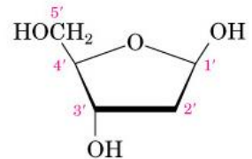
2'-Deossiribosio
