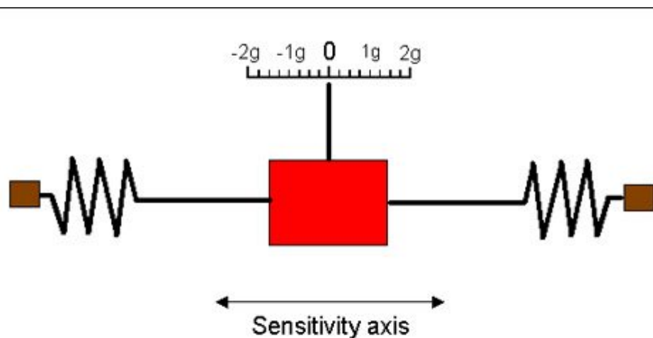
Fig. 1. Schematic structure of an accelerometer
