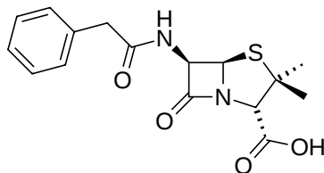
benzil penicillina
