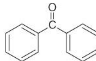
benzofenone
