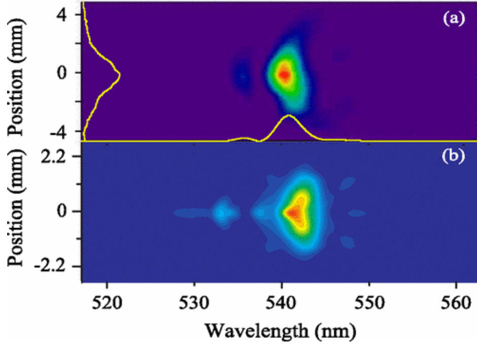
Figure 7.6: Typical FEL spectrum showing a single spike from the experiment (a) and from the Genesis 1.3 simulation (b). The total pulse energy is 300 \mu\text{J} . Taken from [75].
