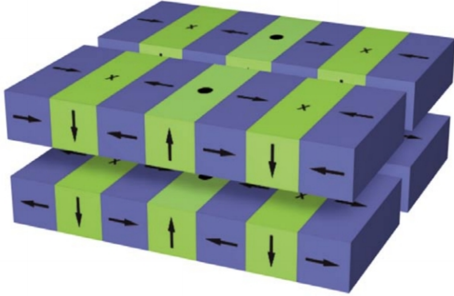
Figure 3.8: Sketch of Apple II block configuration. Each period contains 4 blocks, one for each array. Taken from [24].
