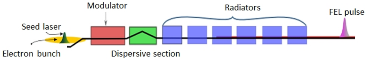
Figure 3.7: Schematic of the FERMI FEL1. The electron beam is sent to the FEL1 line. Electrons interact with the seed laser within the modulator. Here the beam energy is modulated by the laser. FEL radiation is emitted in the radiator at the desired harmonic of the seed. The radiator is composed of 6 Apple II undulators. Taken from [24].
