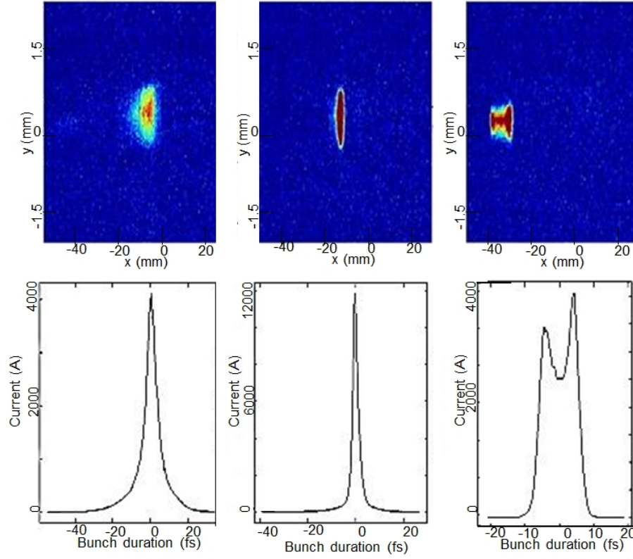
Figure 6.8: On the top: Three images of the electron beam on the spectrometer screen for three different compressions. On the bottom: The corresponding current in the undulator obtained from linac simulations for the same three compression settings used for the measurements shown above (courtesy of J. Wu).
