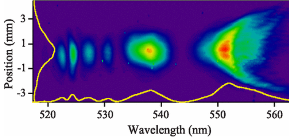
Figure 7.2: Single-shot spectrum acquired with all undulators set at nominal resonance of 540\text{ nm} , with spectrometer entrance slit opened at 100\text{ m} , corresponding to a resolution of 0.17\text{ nm} . The vertical axis represents the non-dispersive dimension at the slit. Taken from [75].
