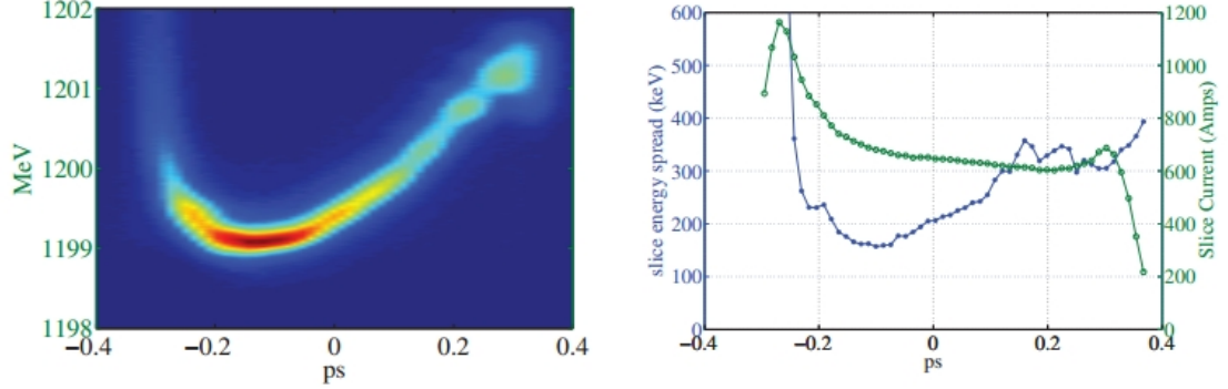
Figure 4.8: Left: longitudinal phase space at the end of the linac. The laser heater and X-band cavity are on and optimized. All the RF sections, with the exception of the last two are set to +30 deg off crest. The vertical axis of the plot on the left is scaled to resolve the residual quadratic chirp. Right: current and energy spread profile in the same linac configuration of the left figure. The energy spread reported here is obtained by screen measurements using a pure chromatic approximation given by equation 2.16. Taken from [126].
