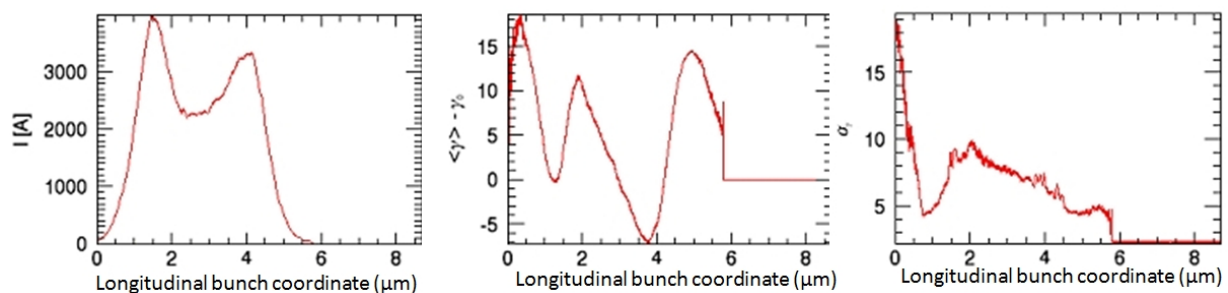
Figure 6.9: Current profile (a), energy profile (b) and energy spread profile (c) of the beam used in start to end simulations. The head of the beam is on the right.
