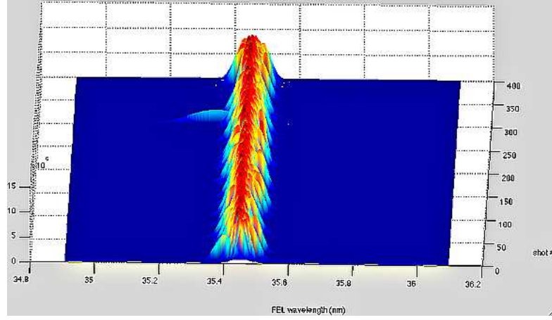
Figure 5.11: Single-shot spectra at 35.4 nm .
