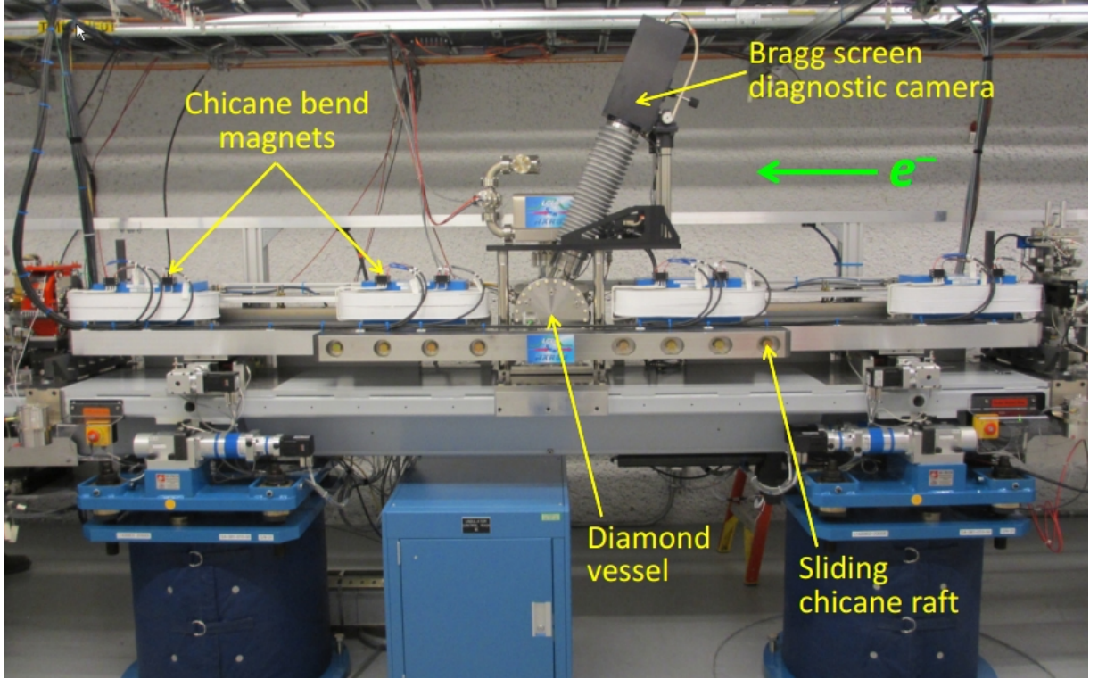
Figure 3.14: Hardware for self-seeding installed on the girder of U16. The chicane for the electron beam is formed by four magnets. The vessel containing the diamond and the diagnostics for the Bragg reflection is installed in the middle of the chicane. Courtesy of P. Emma.
