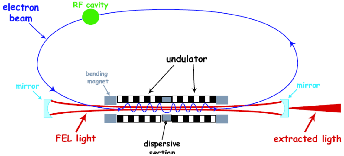
Figure 1.7: FEL oscillator on a storage ring. The radiation produced by the electrons in the undulator is stored in an optical cavity and interacts with the electron beam in the following turns. The undulator can be a single section or, as in the picture, a Klystron composed by two undulators and a dispersive section. Courtesy of F. Curbis.
