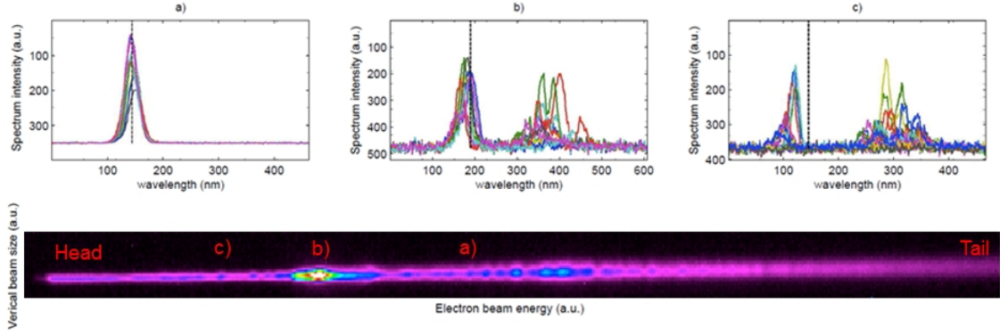
Figure 5.9: FEL power vs. position of the hole observed in the beam energy spectrum. The subplots a, b and c indicate the three series of ten single-shot spectra each collected as the FEL is produced in the three regions of the electron beam identified by the corresponding letters on the electron beam spectrum. Courtesy of E. Allaria.
