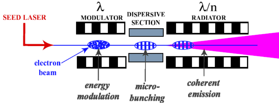
Figure 1.5: Scheme of a FEL working in the HGHG. The electron beam interacts with the seed laser within the modulator. Here the beam energy is modulated by the laser. The energy modulation is converted in a density modulation, at the harmonics of the laser wavelength, in the dispersive section. FEL radiation is emitted in the radiator tuned at the desired harmonic of the seed. Courtesy of F.Curbis.
