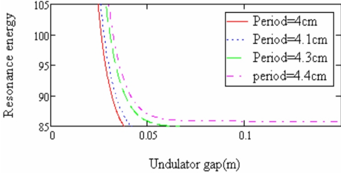
Figure 4.11: Resonance energy in vs. undulator gap. The undulator tunability has been evaluated for different undulator period lengths.
