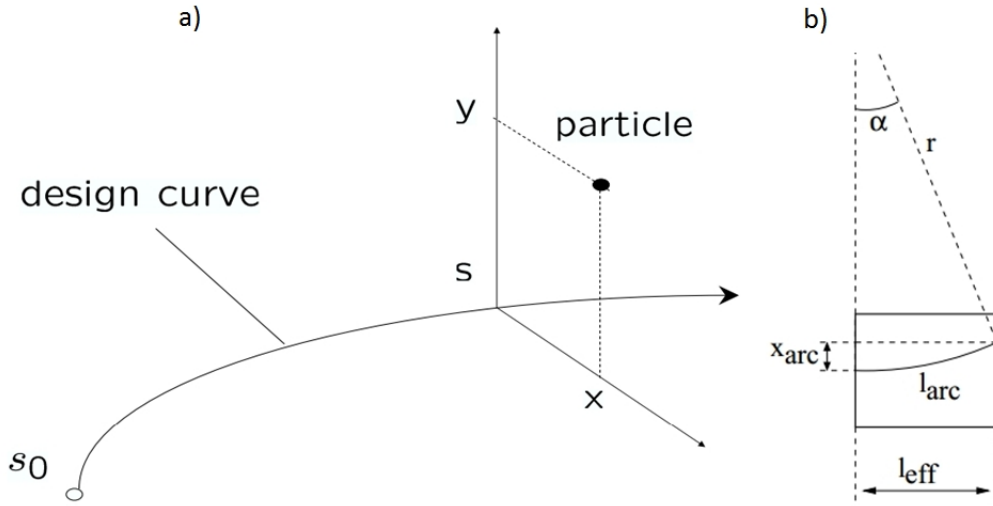
Figure 2.1: a: Design orbit and coordinate system. Taken from [87]. b: Trajectory in a dipole. Taken from [88].
