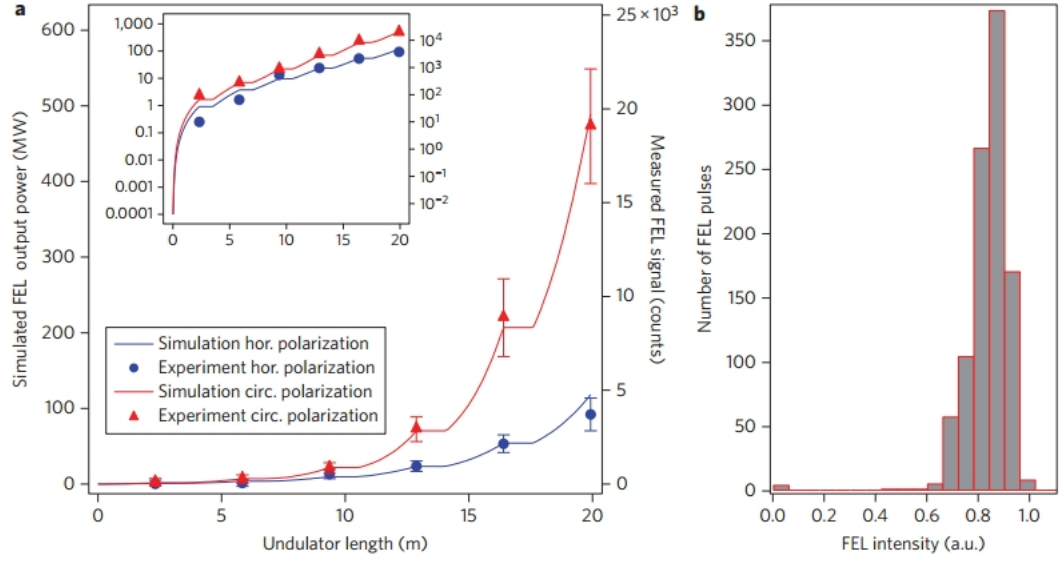
Figure 5.3: Measured FEL intensity at 32.5 nm. a: Measured FEL energy per pulse (symbols, right axis) as a function of the number of undulator sections used in the radiator, and predicted FEL power from numerical simulations [37] (lines, left axis). Data are shown for both circular (red symbols) and horizontal (blue symbols) polarization of the radiator sections. Error bars reflect the statistical distribution of results obtained from several consecutive pulses. In the inset, the same data are reported in a logarithmic scale. b: Typical shot-to-shot distribution of the pulse energy per for 500 consecutive FEL pulses. The quasi-Gaussian distribution characterized by a standard deviation of about 10% reflects shot-to-shot fluctuations in the electron-beam parameters. Taken from [13].
