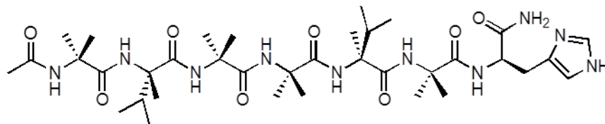
Ac-Aib-L-( \alpha Me)Val-Aib-Aib-L-( \alpha Me)Val-Aib-His-NH 2
