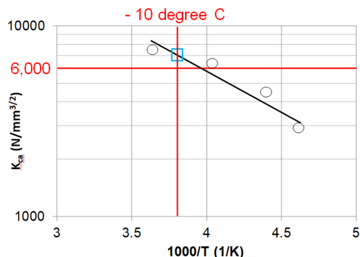
Figure 11 : Example for evaluation of temperature corresponding to the required K_{ca} (1/1/2021)
