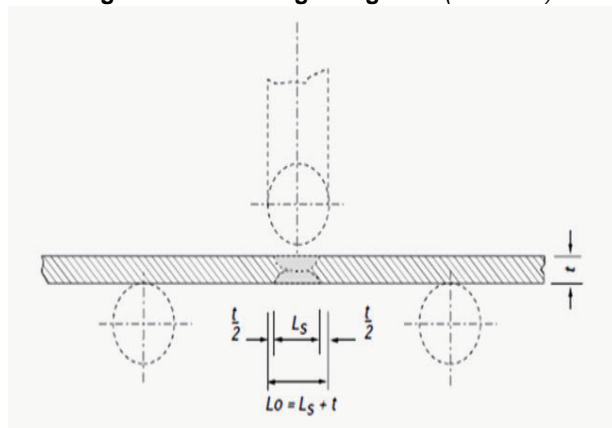
Figure 11 : Bending elongation (1/7/2019)
