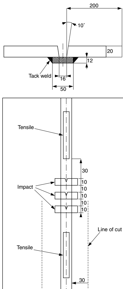
Figure 5 : Deposited metal test assembly (1/7/2019)
