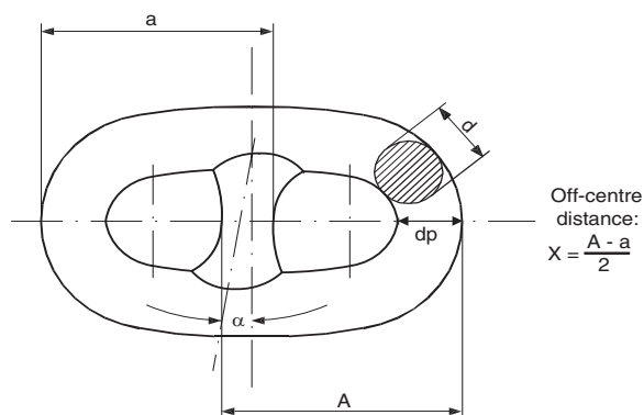
Figure 6 : Manufacturing tolerances
