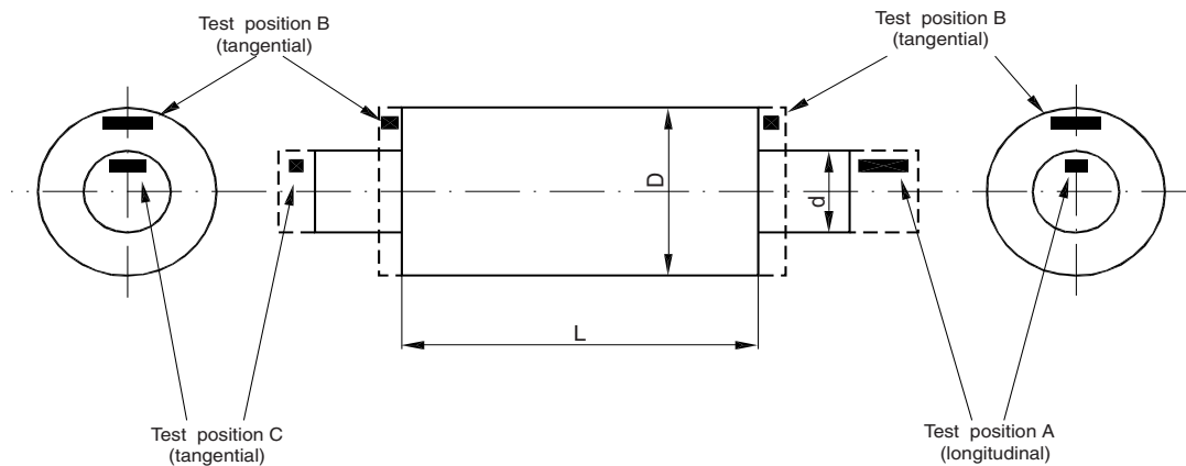
Figure 5 : Pinions
