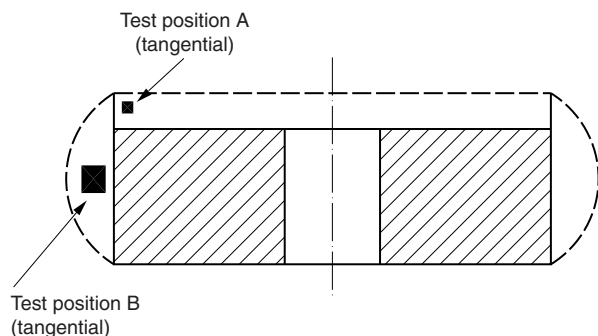
Figure 6 : Gear wheel
