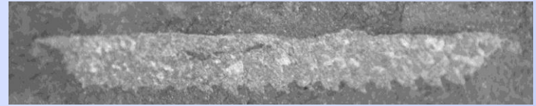
Graptoliti
