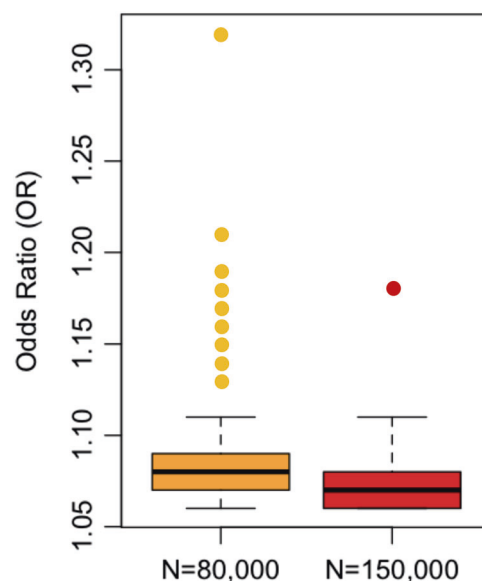
Fig. 2 On average, the largest effect loci are detected first in GWAS. As power increases (typically through increased sample size), smaller effect variants are discovered. Each point represents one of the 128 variants from the 2014 publication of the Psychiatric Genomics Consortium (PGC) Schizophrenia Group. Of the 128 loci, 105 variants were significant associated with schizophrenia (i.e. p < 5 \times 10^{-8} ) in the smaller sample size of approximately 80,000 (yellow). An additional 23 variants reached genome-wide significance using the larger sample size of approximately 150,000 (red, mostly additional control samples)
