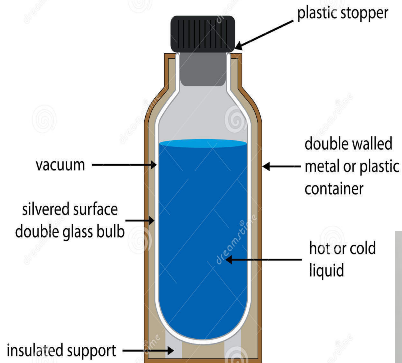
Vacuum or Dewar Flask
