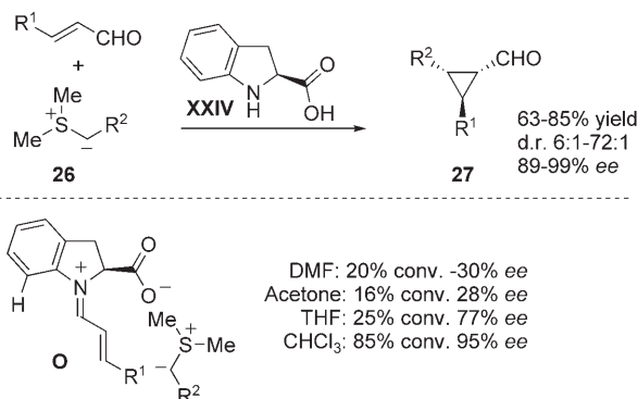
Scheme 34. Organocatalytic cyclopropanation.
