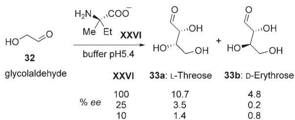
Scheme 43. Primary amino acids as prebiotic asymmetric catalysts.
