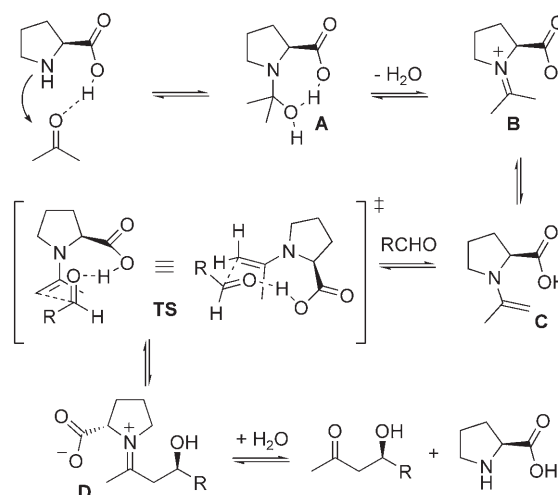
Scheme 5. The proposed mechanism for the direct asymmetric intermolecular aldolization of acetone. The transition state contains a single proline molecule.
