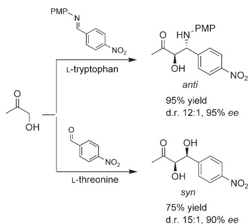
Scheme 44. Primary amines in enamine catalysis.
