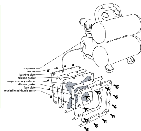
test jig assembly
