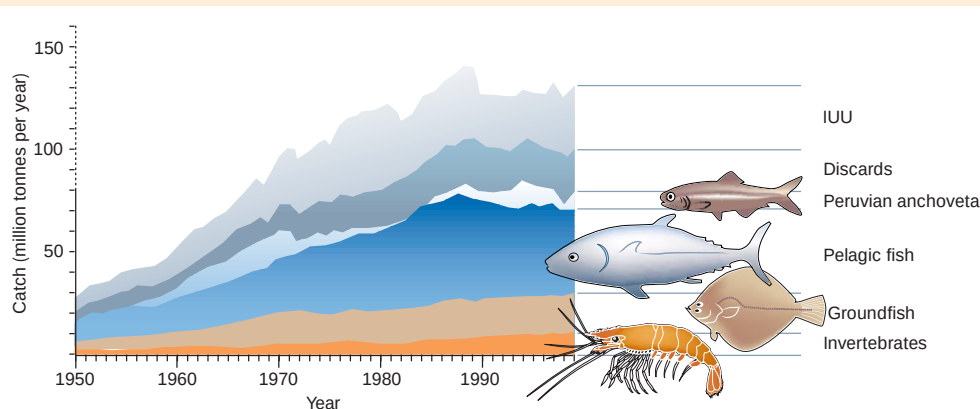
Figure 1 Estimated global fish landings 1950–1999. Figures for invertebrates, groundfish, pelagic fish and Peruvian anchoveta are from FAO catch statistics, with adjustment for over-reporting from China 26 . Fish caught but then discarded were not included in the FAO landings; data relate to the early 1990s 83 were made proportional to the FAO landings for other periods. Other illegal, unreported or unregulated (IUU) catches 65 were estimated by identifying, for each 5-year block, the dominant jurisdiction and gear use (and hence incentive for IUU) 84 ; reported catches were then raised by the percentage of IUU in major fisheries for each 5-year block. The resulting estimates of IUU are very tentative (note dotted y-axis), and we consider that complementing landings statistics with more reliable estimates of discards and IUU is crucial for a transition to ecosystem-based management.
