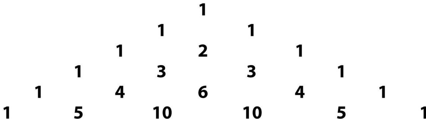
1 Pascal's triangle
