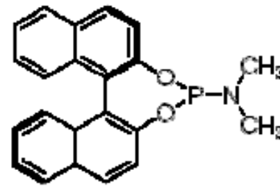
(R)-Monophos
