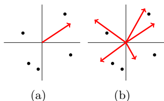
Figure 15.12: (a) : Under-complete representation. There are too few basis vectors to represent the datapoints exactly. (b) : Over-complete representation. There are too many basis vectors to form a unique representation of a datapoint in terms of a linear combination of the basis vectors.
