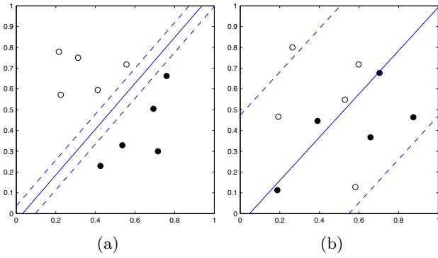
Figure 17.10: The decision boundary p(c = 1|\mathbf{x}) = 0.5 (solid line) and confidence boundaries p(c = 1|\mathbf{x}) = 0.9 and p(c = 1|\mathbf{x}) = 0.1 after 10000 iterations of batch gradient ascent with \eta = 0.1 . (a): Linearly separable data. (b): Non-linearly separable data. Note how the confidence interval remains broad, see demoLogReg.m .
