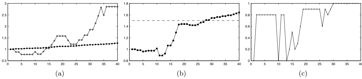
Figure 7.12: (a): Two assets through time – a risky asset whose value fluctuates wildly, and a stable asset that grows slowly. (b): The wealth of our portfolio over time, based on investing with the hope to achieve a wealth of 1.5 at T = 40 . (c): The optimal investment decisions through time, with 1 corresponding to placing all wealth in the safe asset and 0 placing all the money on the risky asset.
