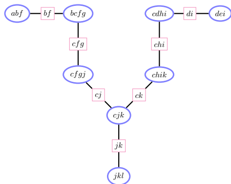
Figure 6.9: Junction tree formed from the triangulation fig(6.8f). One may verify that this satisfies the running intersection property.
