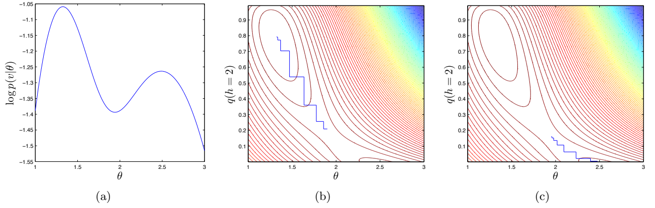
Figure 11.2: (a) : The log likelihood for the model described in example(11.2). (b) : Contours of the lower bound \tilde{L}(q(h = 2), \theta) . For an initial choice \theta = 1.9 , successive updates of the E (vertical) and M (horizontal) steps are plotted, with the algorithm converging to the global optimum maximum likelihood setting for \theta . (c) : Starting at \theta = 1.95 , the EM algorithm converges to a local optimum.
