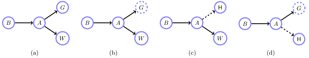
Figure 3.3: (a): Mr Holmes' burglary worries as given in [236]: (B)urglar, (A)larm, (W)atson, Mrs (G)ibbon. (b): Mrs Gibbon's uncertain evidence represented by a dashed circle. (c): Virtual evidence or the replacement of unreliable evidence can be represented by a dashed line. (d): Mrs Gibbon is uncertain in her evidence. Holmes also replaces the unreliable Watson with his own interpretation.
