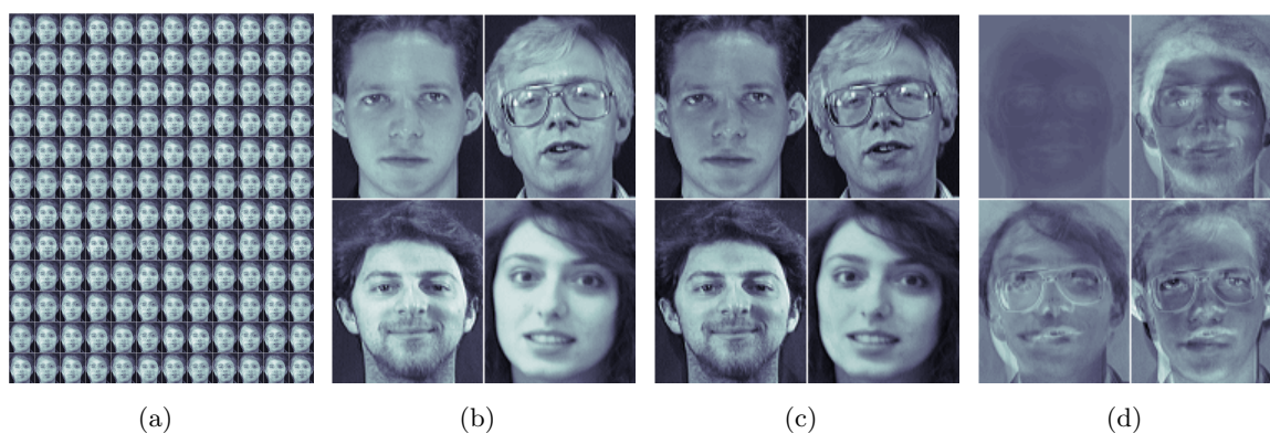
Figure 15.15: (a): Training data, consisting of a positive (convex) combination of the base images. (b): The chosen base images from which the training data is derived. (c): Basis learned using conditional PLSA on the training data. This is virtually indistinguishable from the true basis. (d): Eigenbasis (sometimes called ‘eigenfaces’).
