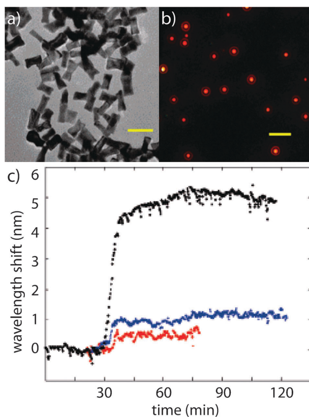
Fig. 12 A single particle localized surface plasmon resonance (LSPR) assay for biomolecular detection. (a) Electron micrographs of gold nanorods. (b) Optical dark-field scattering microscopy of gold nanorods. (c) Real-time measurement of the binding of streptavidin and biotin by monitoring the light scattering spectra of a single biotin-conjugated gold nanorod. Black, blue, and red curves represent the spectral shift over time when biotin-conjugated gold nanorods were incubated in 130 nM, 10 nM and 1 nM streptavidine in PBS. The gold nanorods showed a sensitivity of streptavidin detection down to 1 nM. Figures adapted with permission from ref. 219. Copyright 2008 American Chemical Society.
