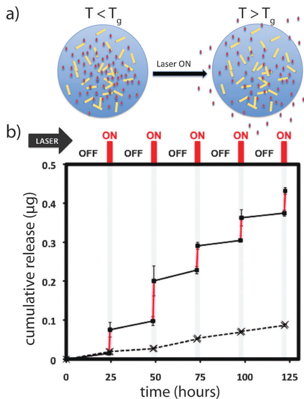
Fig. 22 (a) Illustration demonstrating the use of gold nanoparticles in a composite material to enable light-triggered drug delivery. Gold nanorods distributed in a polymeric microsphere matrix act as localized nanoheaters upon light irradiation. Gold nanorods absorb light and convert it into heat which changes the polymeric matrix from a glassy state to a rubbery state and allowing enhanced drug diffusion and release. (b) Experimental results showing drug release as a function of laser irradiation cycles/duration for a microsphere matrix containing gold nanorods. Squares: with laser; X: no laser. Laser \lambda_{\text{max}} = 808 nm; T_g = glass transition temperature. 407 Panel (b) is adapted with permission from ref. 407. Copyright 2011 American Chemical Society.
