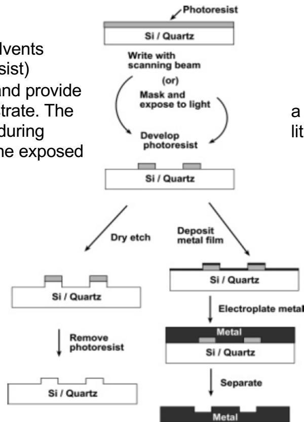
Figure 1. Schematic illustration of the fabrication of topographically patterned surfaces in hard materials by conventional photolithography and electroplating.
