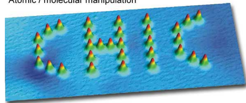
Example 1: Individual Cu atoms on Cu(111). Size: 25 x 8 nm 2 .
