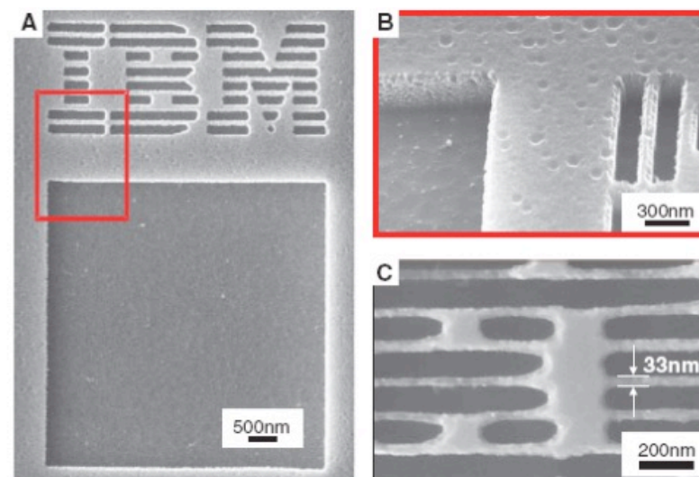
Fig. 3. Pattern transfer into silicon. (A) SEM image of the pattern shown in Fig. 2 transferred 400 nm deep into silicon. (B) Tilted view of the structure indicated by the red box in (A) . (C) Zoom into a similar structure as shown in (A) but written at half the pixel pitch. The smallest lines fabricated in silicon had a width of \sim 30 nm.
